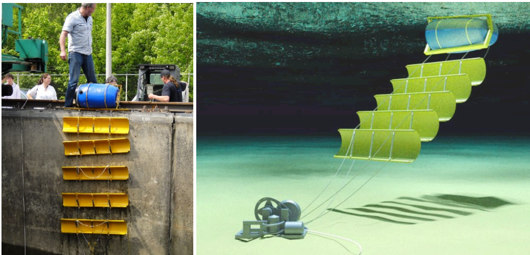
Figure 20 Slowmill being tested at the Delta flume facility of Deltares in 2011
