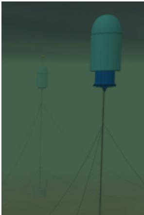
Figure 23 Symphony looks like the Archimedes Wave Swing, but houses an innovative linear power take off system using an air pressure chamber and sliding bellow frames.
