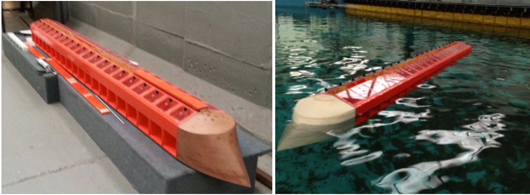
Figure 25 KNSwing being tested at the Hydrodynamic Marine Research Centre Cork (HMRCC), Ireland as part of the MaRINET programme.
