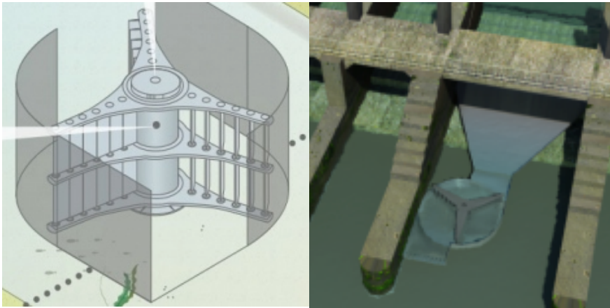
Figure 15 Left: Schematic of the Oryon Watermill, and right: installed in the sluice gate in Ulf, in the Oude IJssel
