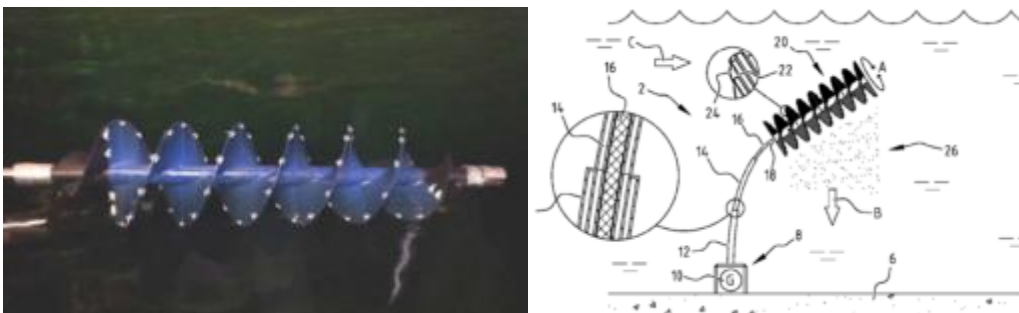
Figure 18 Hydromine model tested at MARIN in 2014 and illustration for seabed mounted solution.
