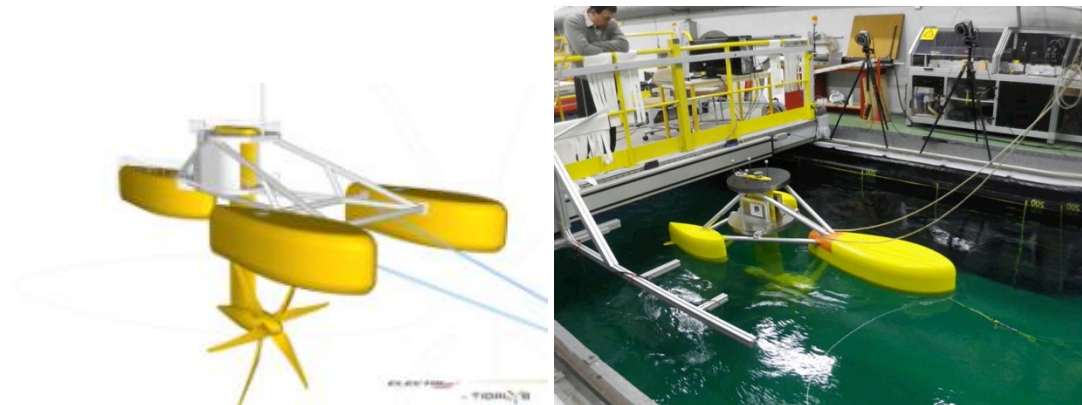
Figure 10 Tidalys counter-rotating turbine. Right: tests at IFREMER, Boulogne sur Mer, France.
